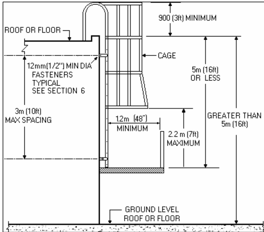
FIG. 3: Typical Steel Access Ladder – Elevated Access General Arrangement – Cage Required for Wide Landings [Ref. Section 5.1.2]
